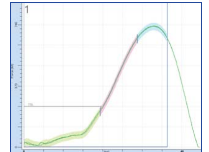
Crimp Force Signature
